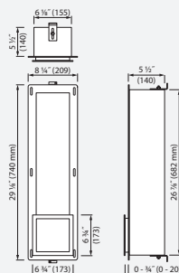
TCL-1 | Toilet paper storage for 6 rolls
