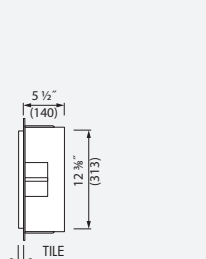
Depth 5 1/2" (140 mm)
