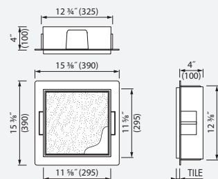
Depth 4" (100 mm)
