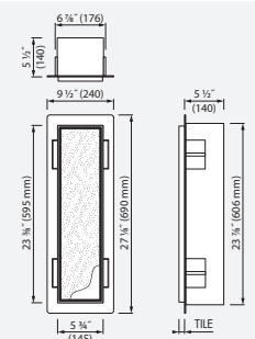
TCL-11 | Built-in waste container & wall niche
