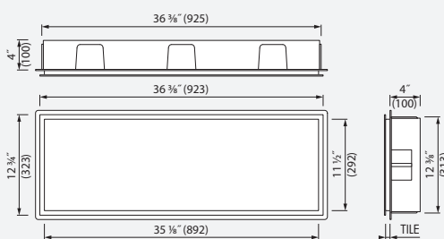
36" x 12" x 4" | 90 x 30 x 10 cm
