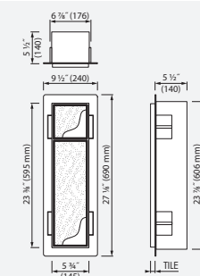
TCL-10 | Built-in toilet brush holder & paper holder
